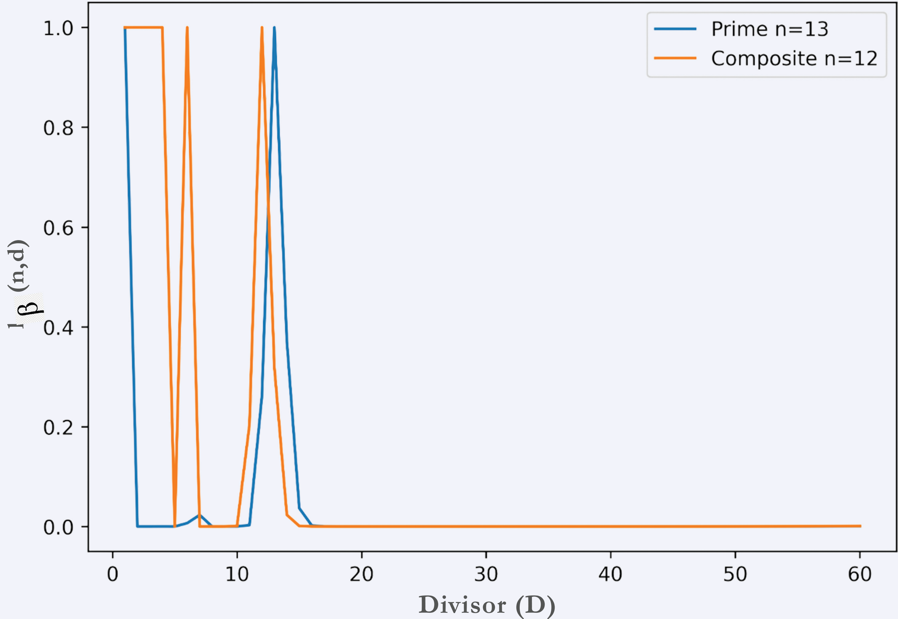
Figure 4: Prime vs Composite overlay, \beta=20
