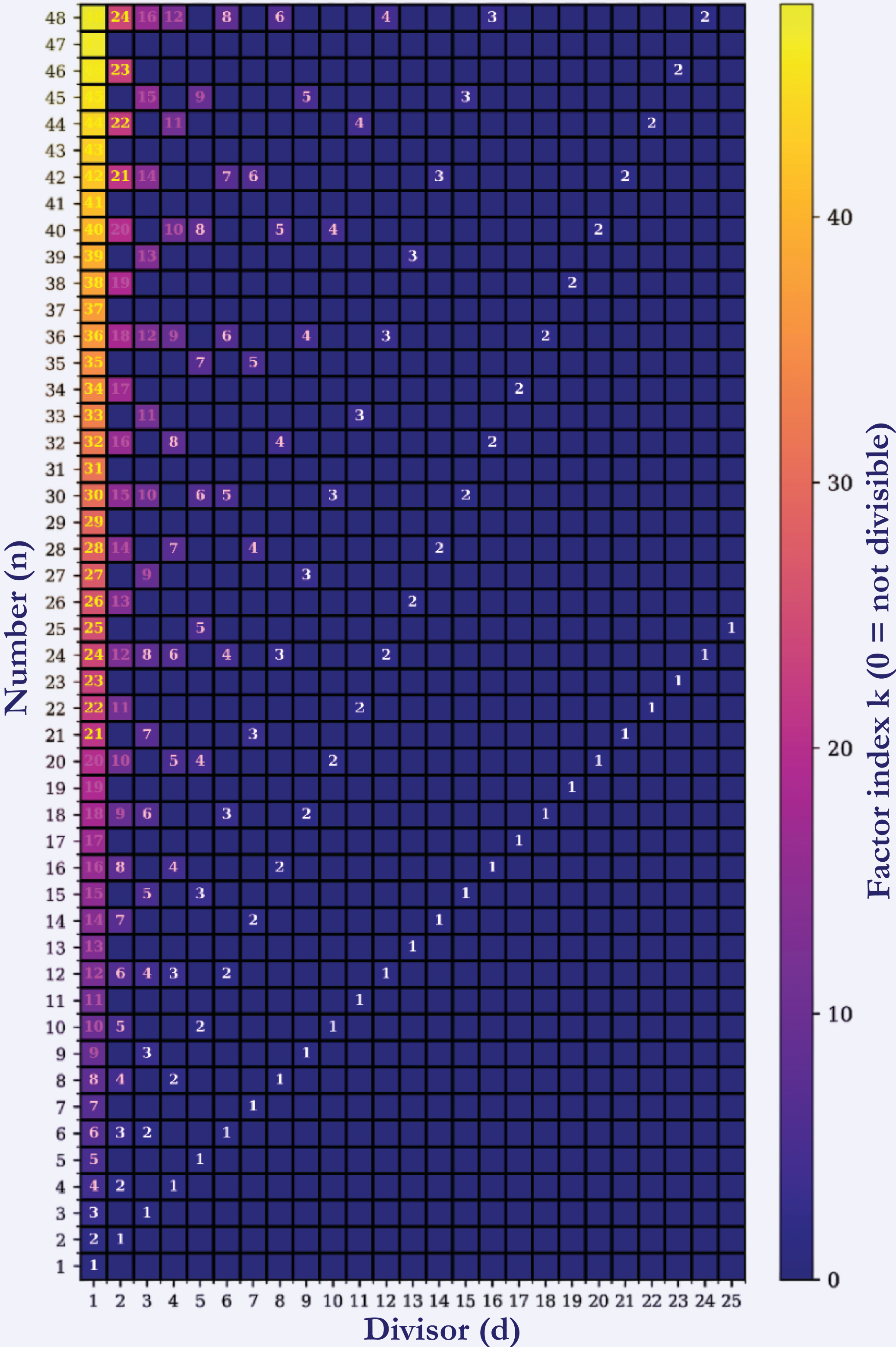
Figure 2. Counting Divisor Grid for integers 1–48.
